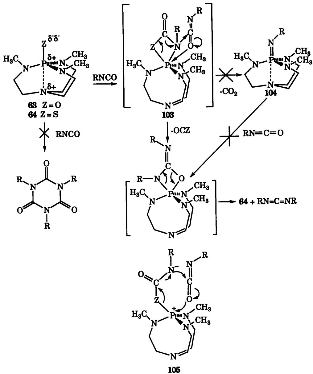
Scheme 3
