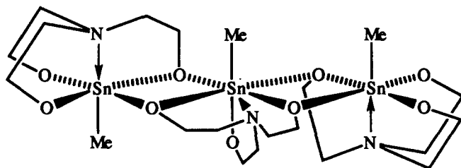
120 (R = Me)
